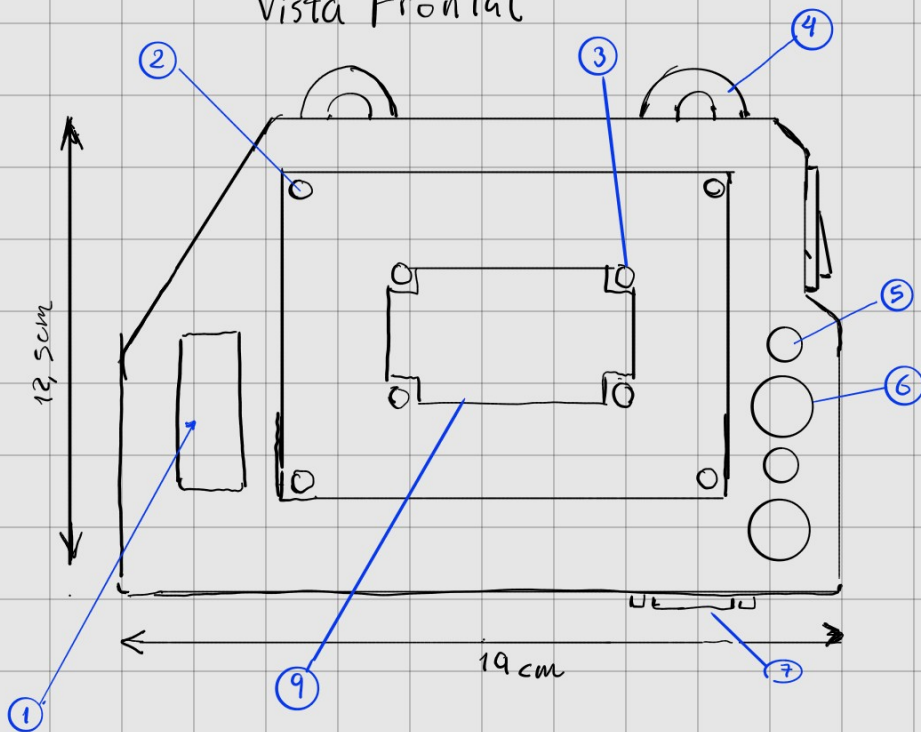
Vista Frontal
